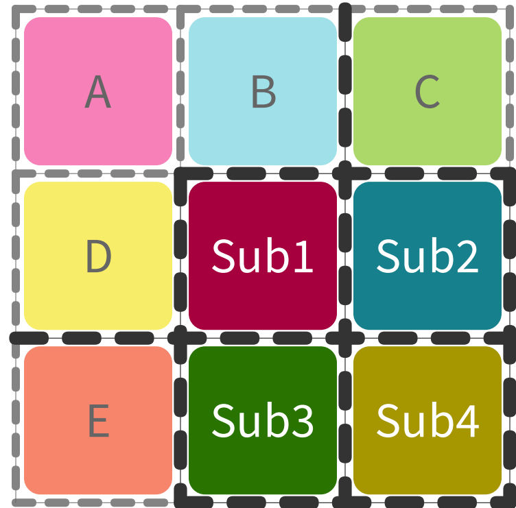
Subgrid
